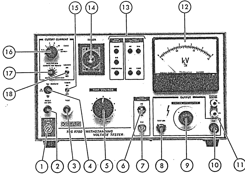
Figure 4.1 Model TOS8750
